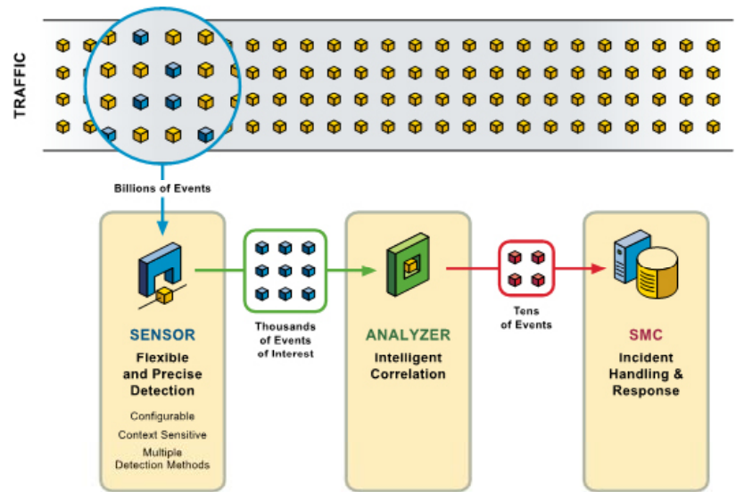
Figure 3. Incident Handling in StoneGate IPS
