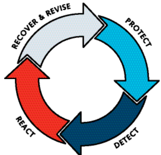
Figure 1: Security Model
