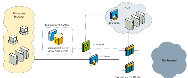
Figure 2: StoneGate Security Solution
