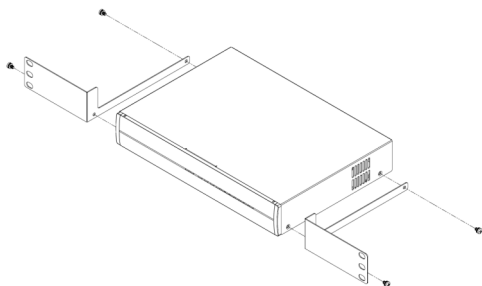
ILLUSTRATION 3 Attaching the Brackets to the Appliance
