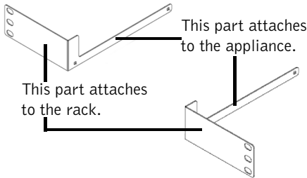
ILLUSTRATION 1 Bracket Parts
