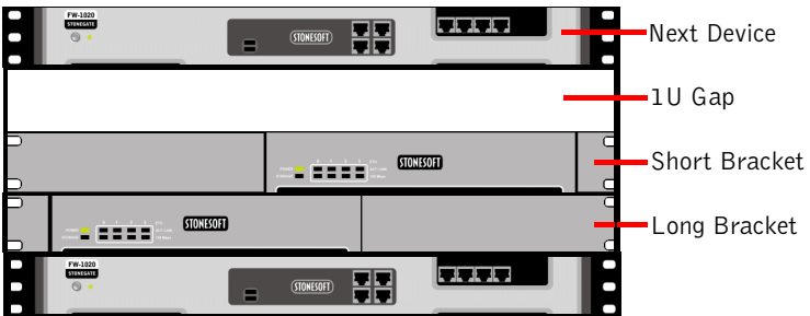
ILLUSTRATION 3 Correct Rack-Mounting Setup
