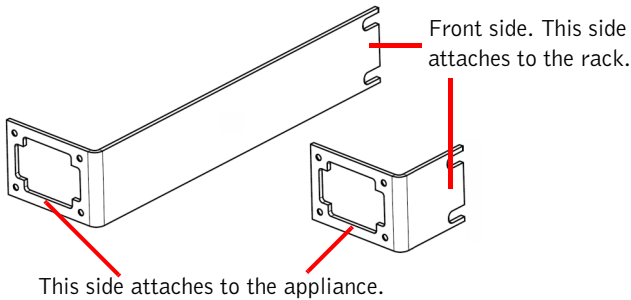
ILLUSTRATION 1 Parts Included
